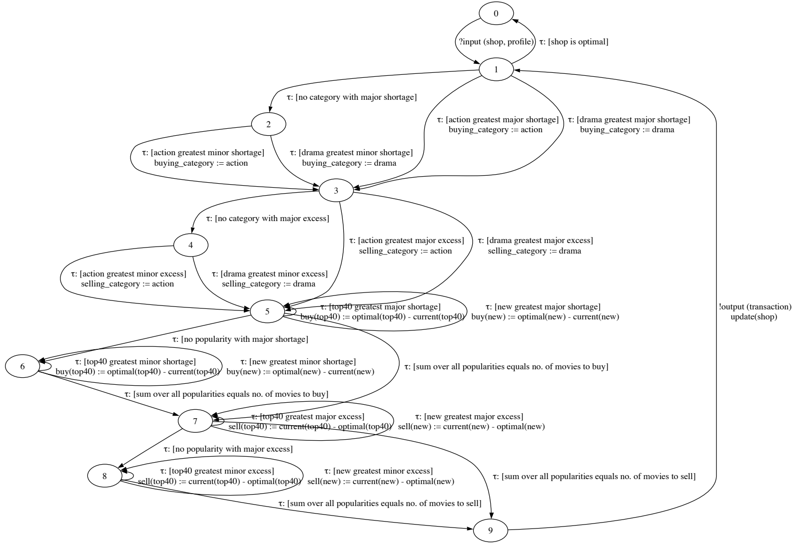
Figure 6: The Symbolic Transition System for the Blockbuster case
