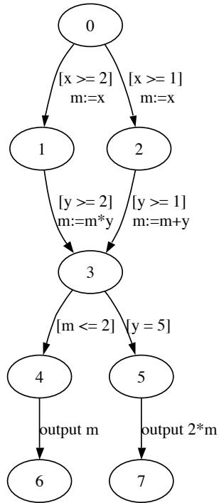
Figure 12: The CFG of a correct implementation of the specification
